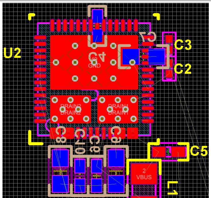
Figure 45. Bottom View Layout
