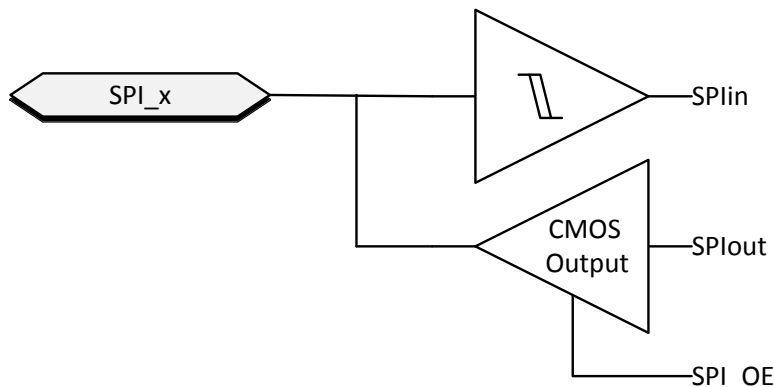
Figure 24. SPI buffer
