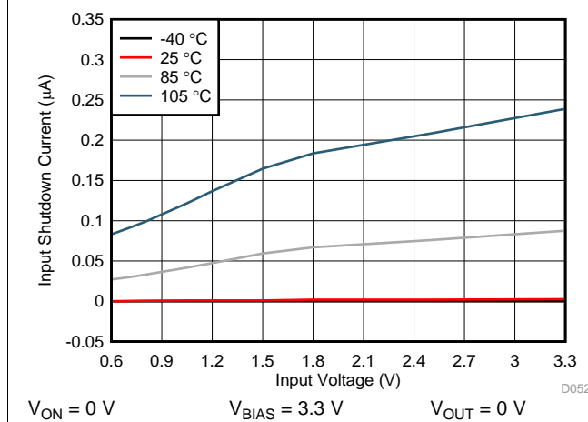
Figure 3. Input Shutdown Current vs Input Voltage
