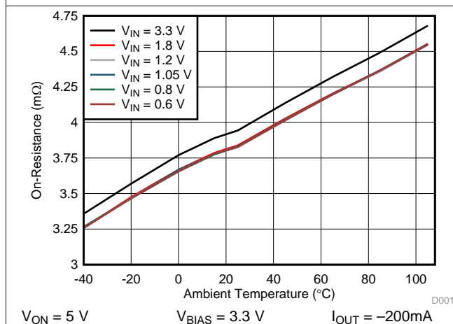
Figure 5. On-Resistance vs Ambient Temperature
